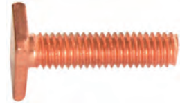
234316 Fixed Contact Servicing: TPB136, TPB138, TPB142, TPB143, TPB150 Total length 26.75, Thread size M6
