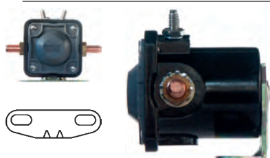
139858 Solenoid Replacing: 2095606, 1658883, SAZ4201J, 15-66, 15-5C, 15-288, 1114537, 1114206 12 V, 100 Amp, Intermittent load 600 Amp., B+ M8, Kl. 50 M5, OD 41.90, Total length 63.45, Height/B+ 18.75, Width/kl. 50 12.75, Coil bolt M8, Coil bolt 2 18.55, No./terminals 4 Insulated return.
