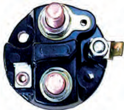
136055 Solenoid Cap Servicing: 63221300, 63221330, 63221535, 63601007, 85540461 OD 50.50, No./terminals 4 HC-CARGO 134862.
