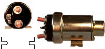
231810 Solenoid 24 V, 200 Amp, Intermittent load 800 Amp., B+ M8, Kl. 50 6.30, OD 44.90, OD/cover 47.45, Total length 114.55, Height/B+ 11.10, Width/kl. 50 11.55, Coil bolt M8, Coil bolt 2 11.40, Seconds 5, No./terminals 3
