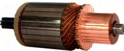
234107# Armature
