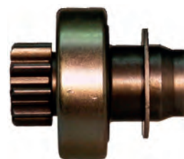
139898# Drive Replacing: 183776, 182243 Servicing: D9E108 ID 12.20, OD 26.75, OD/housing 47.85, Total length 54.75, Splines A 9, No./teeth 10, Rotation CR
