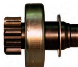
139905 Drive Replacing: 594251, 186321 Servicing: D9R142 ID 12.00, OD 31.90, OD/housing 54.40, Total length 61.30, Splines A 9, No./teeth 10, Rotation CR
