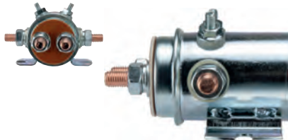
333005 Solenoid 24 V, 75 Amp, Intermittent load 150 Amp., Total length 79.60, No./terminals 6 Coil resistance 16 Ohms. N.C. contact: 60/60 A.
