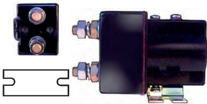
138685 Solenoid 24 V, 100 Amp, B+ M8, Total length 93.80, Height/B+ 20.25, Coil bolt M8, Coil bolt 2 20.10, No./terminals 4 Silver contact.
