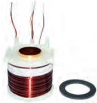
138939 Solenoid Coil Servicing: 228000-5641 24 V, ID 21.00, OD 46.70
