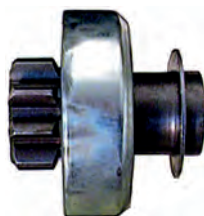
139320 Drive Replacing: 187428 Servicing: D7E2 ID 11.00, OD 25.00, OD/housing 46.00, Total length 43.00, Splines A 5, No./teeth 9, Rotation CR
