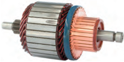
137069 Armature
