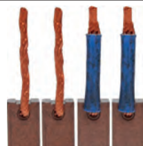
140336 Brush Set Replacing: TAJ101 12 V, Length 16.00, Lead length 36.50, Height 11.00, Thickness 7.00
