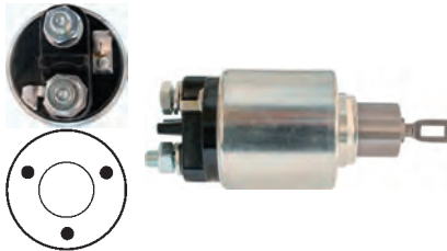
139075 Solenoid
