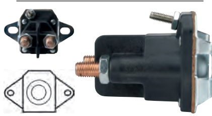
231526 Solenoid 12 V, 80 Amp, B+ 5/16"-24, Kl. 50 M4, OD 55.85, Total length 55.15, Height/B+ 9.50, Width/kl. 50 10.20, Coil bolt 5/16"-24, Coil bolt 2 9.50, No./terminals 3 Relay w/ 1/4" B+: HC-CARGO 234070.
