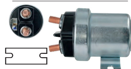
231809 Solenoid 12 V, 200 Amp, Intermittent load 800 Amp., B+ M8, Kl. 50 6.30, OD 45.00, OD/cover 47.30, Total length 104.65, Height/B+ 11.20, Width/kl. 50 11.60, Coil bolt M8, Coil bolt 2 11.50, Seconds 5, No./terminals 3
