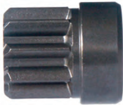
134237# Dp Gear ID 12.00, OD 25.10, Height 32.35, No./teeth 9
