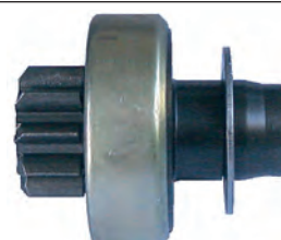
230353 Drive Replacing: NE957, 594303, 187567 Servicing: D7R17, D7R42, D7RP82 ID 12.00, OD 27.95, OD/housing 47.60, Total length 54.85, Splines A 10, No./teeth 10, Rotation CR
