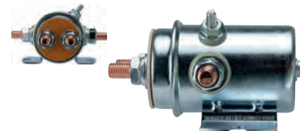
333015 Solenoid 24 V, 50 Amp, Intermittent load 50 Amp., Total length 86.70, No./terminals 5 Coil resistance 60 Ohms. N.C. contact: 30/30 A.
