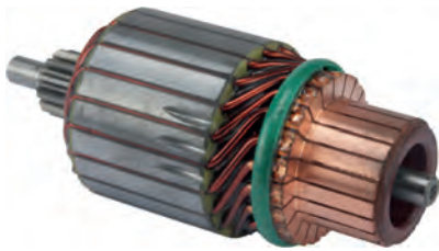
236958 Armature
