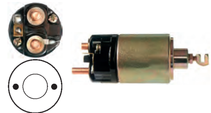
130814 Solenoid
