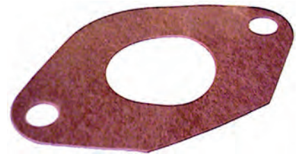
136276 Gasket Servicing: M50 ID 28.00, ID/mount. hole 8.15, Length 80.65, Thickness 0.30, Width 54.00
