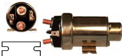
231808 Solenoid 24 V, 200 Amp, Intermittent load 800 Amp., B+ M8, Kl. 50 6.30, OD 45.15, Total length 114.90, Height/B+ 11.20, Width/kl. 50 11.75, Coil bolt M8, Coil bolt 2 11.20, Seconds 5, No./terminals 4
