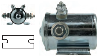
235443 Solenoid 24 V, 100 Amp, Intermittent load 200 Amp., Seconds 5, No./terminals 4 Silver contact. Insulated return.
