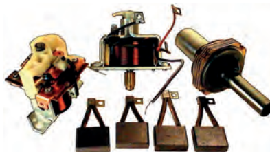
134010 Repair Kit Servicing: 0001415016 For FKB-24 V earthed. Includes: Clutch: HC-CARGO 130317. Solenoid: HC-CARGO 130304, 133554. Brush set: HC-CARGO BSX1314.
