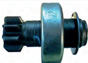
139318 Drive Replacing: 594034, 184795 Servicing: D6RA17, D6RA19, D6RA27, D6RA29, D6RA34, D6RA50, D6RA54, D6RA60 ID 12.00, OD 29.65, OD/housing 47.65, Total length 66.70, Splines A 9, No./teeth 9, Rotation ACR
