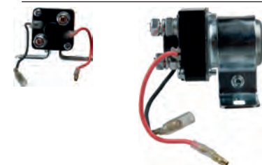
333007 Solenoid 24 V, OD 67.60, Total length 65.00, No./terminals 4
