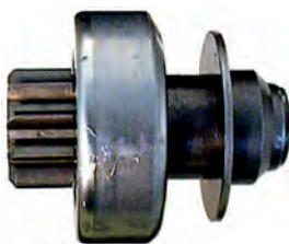
138208 Drive Replacing: 180719 Servicing: D11E272 ID 12.00, OD 27.70, OD/housing 53.50, Total length 65.45, Splines A 9, No./teeth 10, Rotation CR
